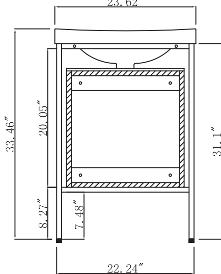
Front view 23.62"
