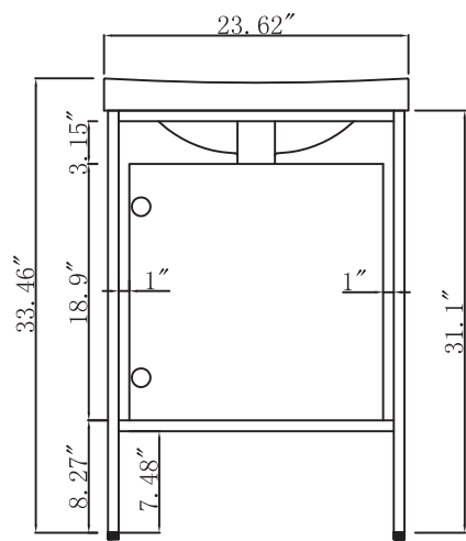
Front view 23.62"
